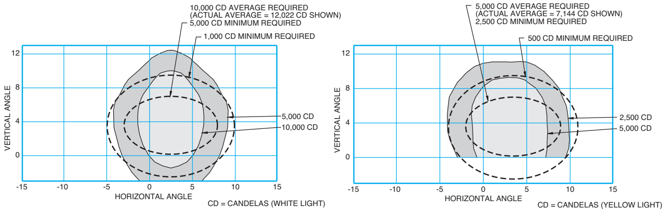
L-850C Inset Runway Edge Light – White
