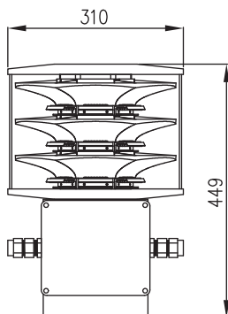
DUAL BEACON FRONT VIEW
