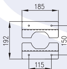
FIXING DETAILS
