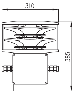
BEACON FRONT VIEW
