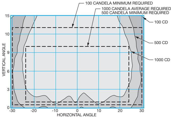
L-852G Runway Guard Light-Yellow
