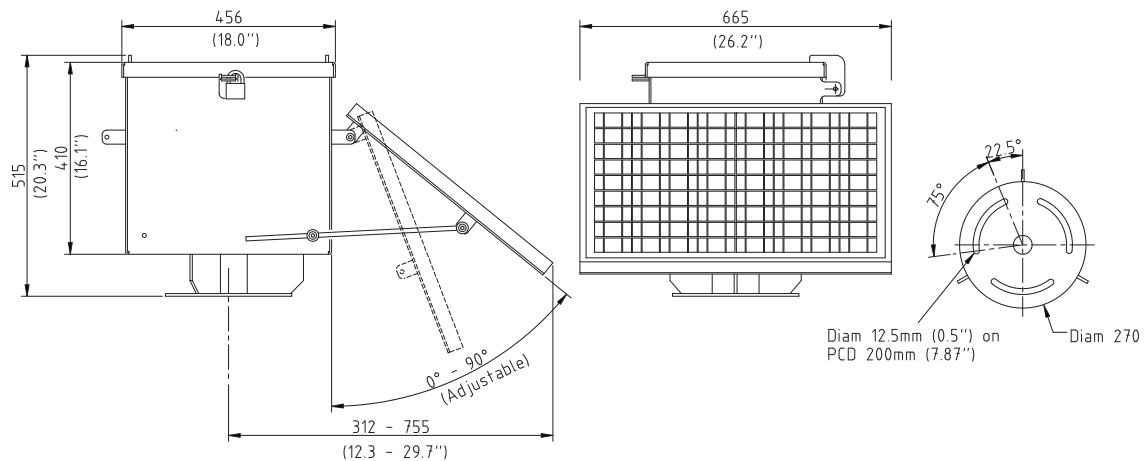
LD-PS-40 40watt bridge light power supply
