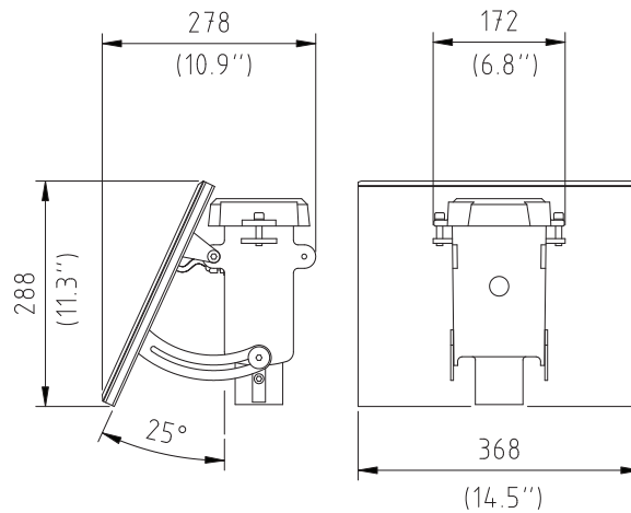
BL-PS-10 10watt bridge light power supply
