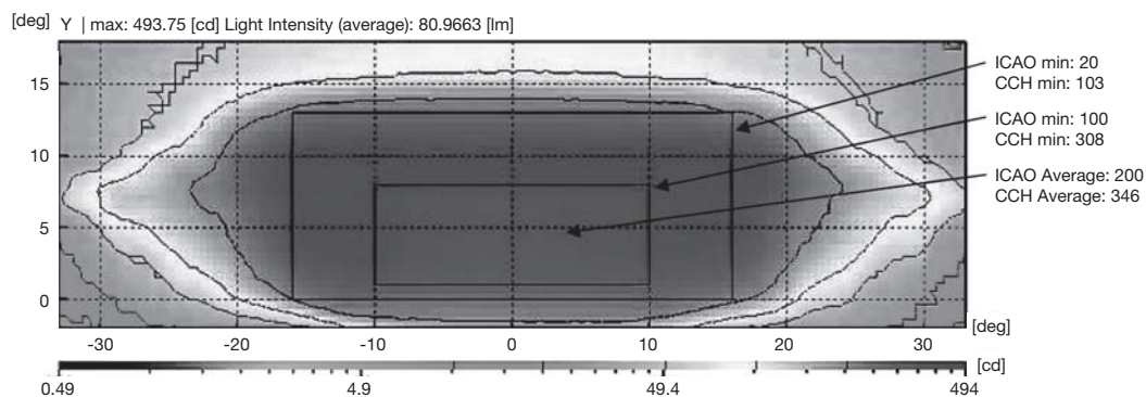
Stopbar, Light Distribution FAA
